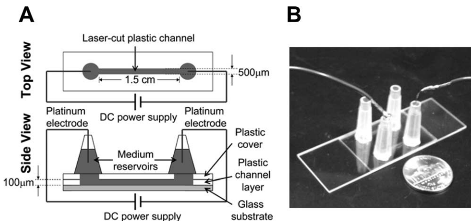
FIGURE 3. Microfluidic chamber for visualization of cell migration in an applied electric field. A , Microfluidic system is illustrated for studying cell migration in an applied electric field. B , An image of the microfluidic system. Two identical channels were configured side-by-side in a single device and can be used for migration studies separately. A nickel was placed next to the device as a scale reference.
